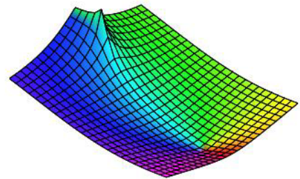
\left|\log\left[\frac{1}{z} \log\left(\frac{1}{1-z}\right)\right]\right|
